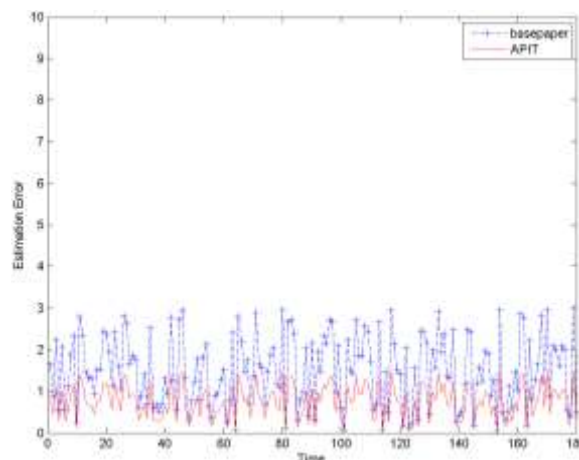
Figure:7 Estimation Error with Respect to time compared with Base paper (blue) [12] and Proposed work APIT scheme (red).
