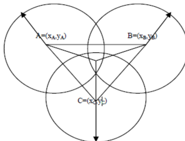
Figure 5: Position Approximation Algorithm
